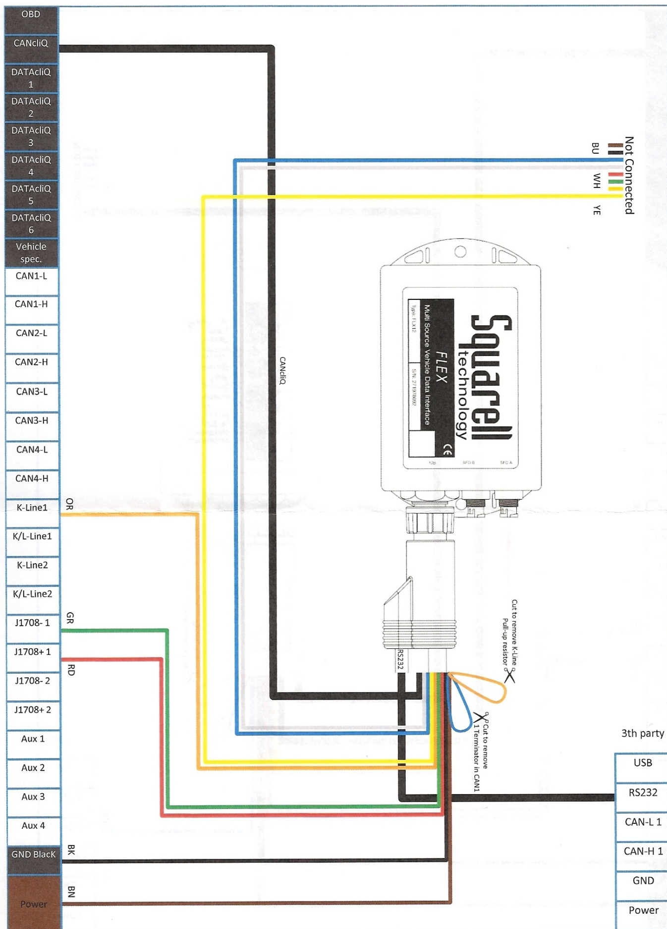
FLX12 FLEX – CANcliQ cable – RS232 output
